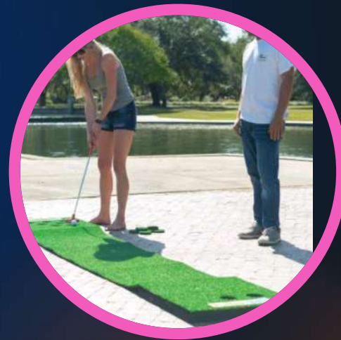
GOLF PONG
